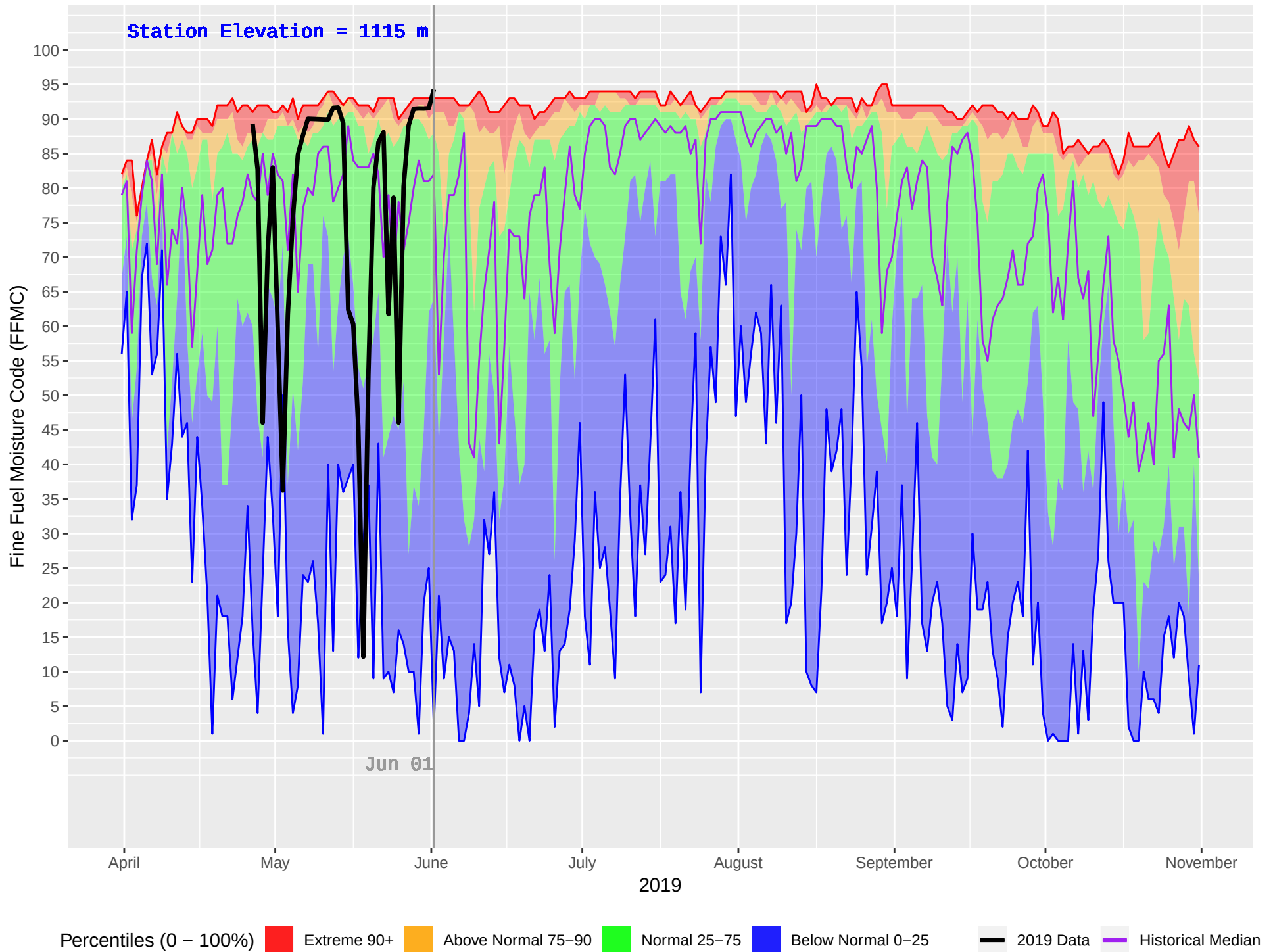
SICAMOUS (882) : Historical (2004–2018) and Current (2019) Daily Fine Fuel Moisture Code (FFMC)
