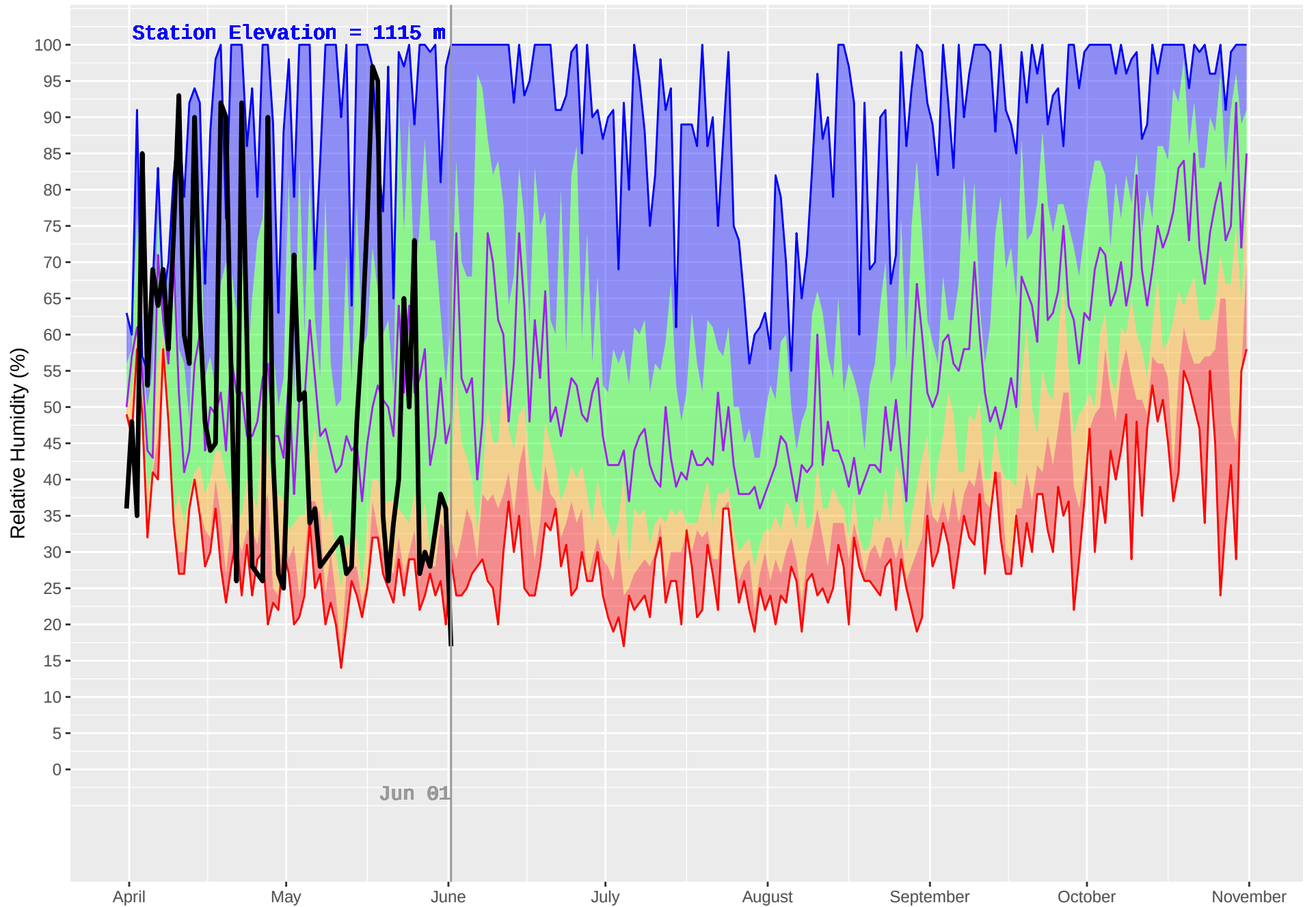
SICAMOUS (882) : Historical (2004–2018) and Current (2019) Daily Relative Humidity
