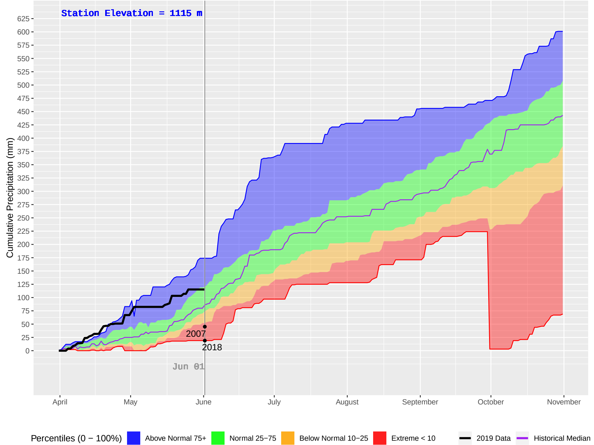
SICAMOUS (882) : Historical (2004–2018), Current (2019) Daily Cumulative Precipitation
