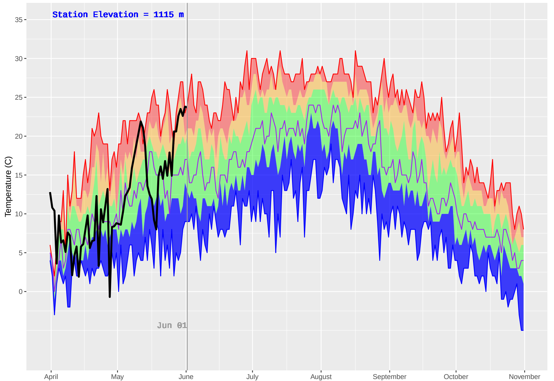
SICAMOUS (882) : Historical (2004–2018) and Current (2019) Daily Temperature
