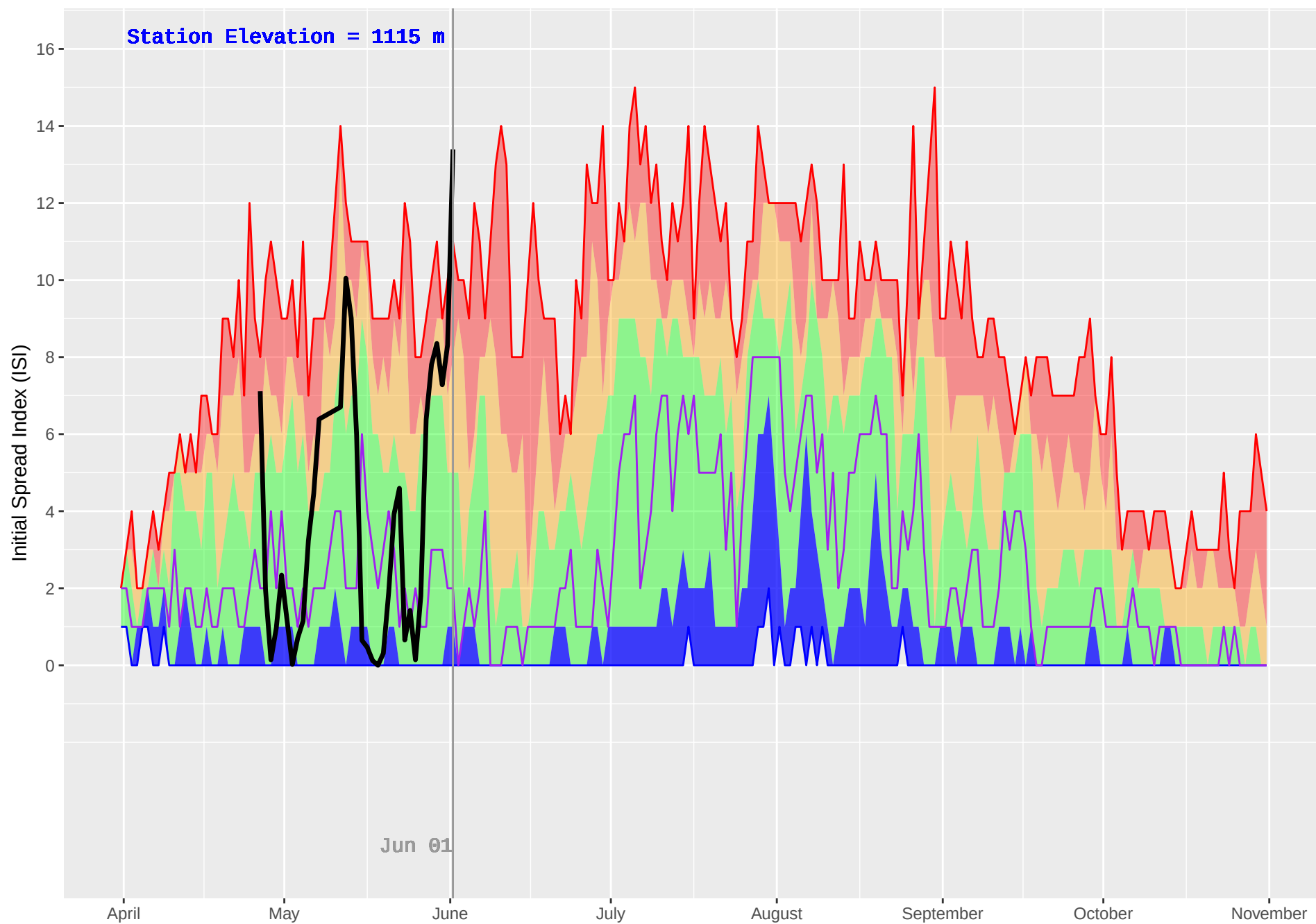
SICAMOUS (882) : Historical (2004–2018) and Current (2019) Daily Initial Spread Index (ISI)
