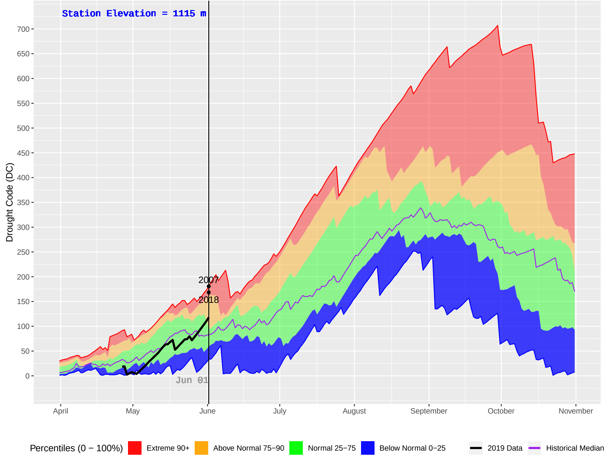
SICAMOUS (882) : Historical (2004–2018) and Current (2019) Daily Drought Code (DC)
