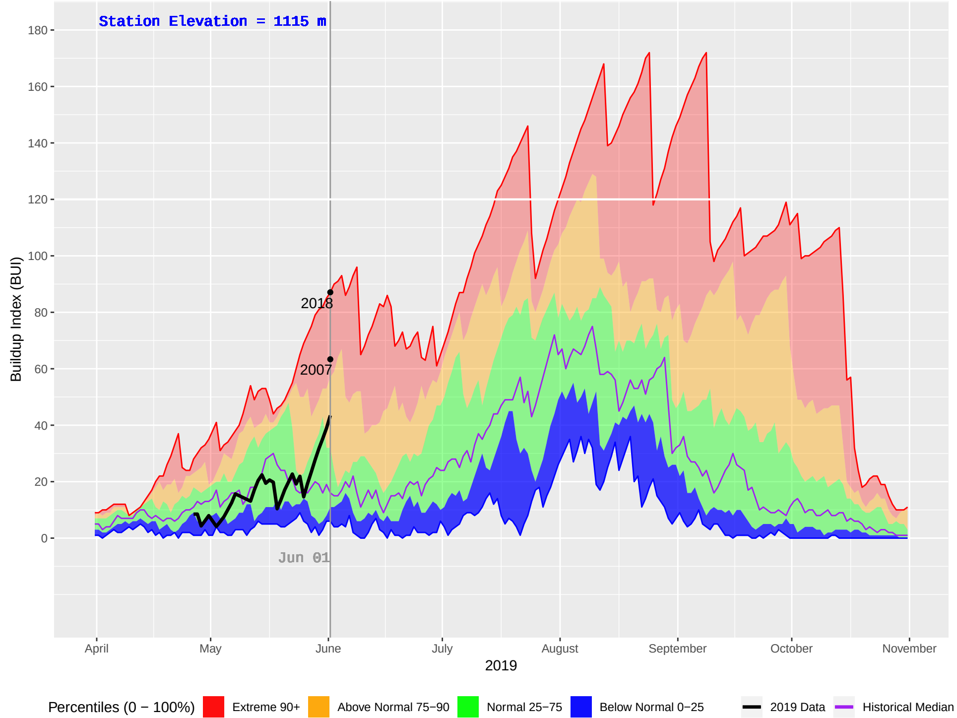
SICAMOUS (882) : Historical (2004–2018), Current (2019) Daily Buildup Index (BUI)
