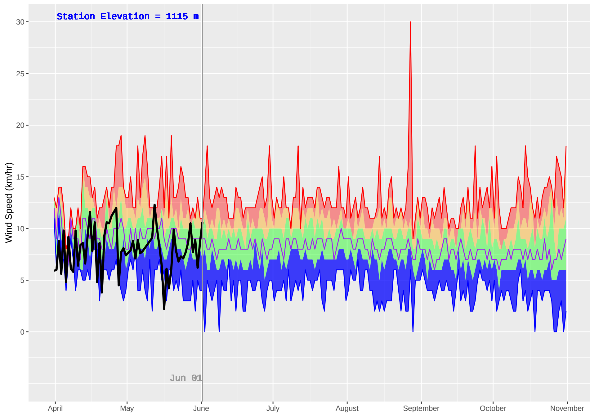
SICAMOUS (882) : Historical (2004–2018) and Current (2019) Daily Wind Speed
